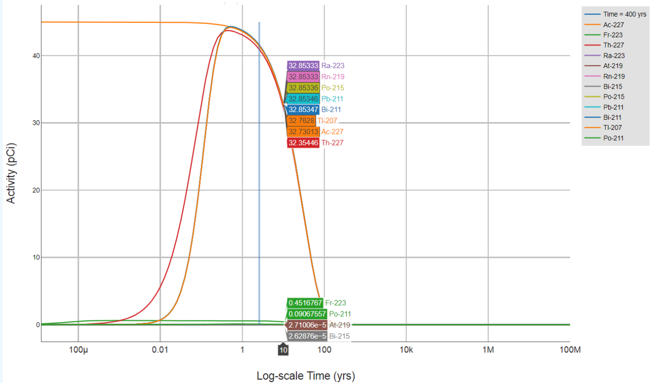
Decay over time for Ac-227 (A 0 = 45 pCi)
