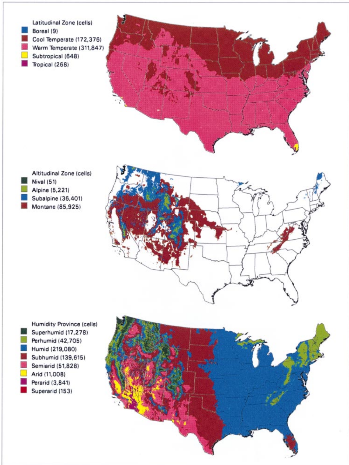
Figure 4 Life zones of the United States aggregated by (a) latitudinal zones (b) altitudinal zones (white is the basal zone), and (c) humidity provinces.
