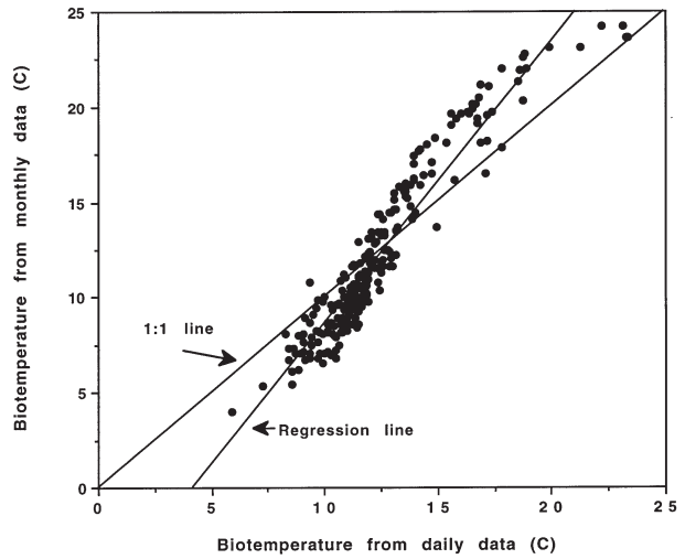
Figure 2 Relation between mean annual biotemperature ( T_{bio} ) based on daily station data and that based on monthly surface data ( n=241 , r^2=0.96 ; see text for further details).
