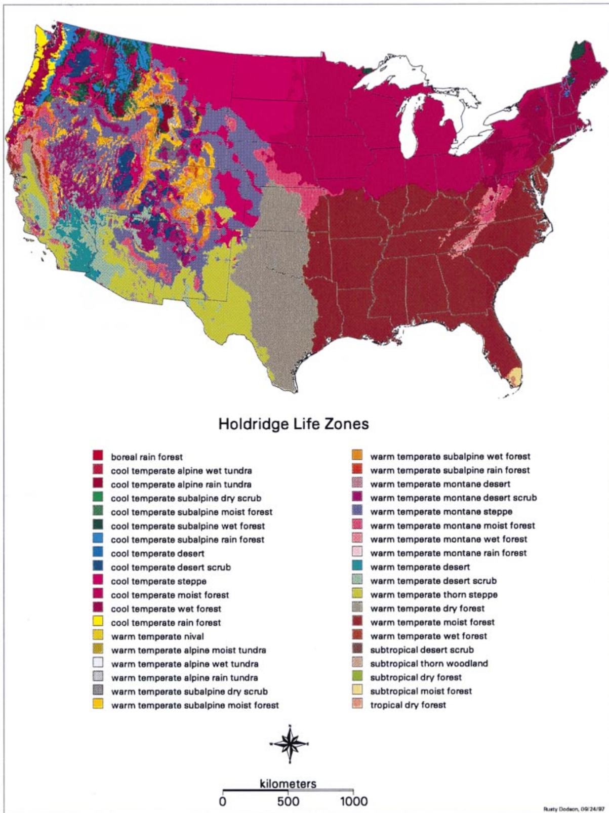
Figure 3 Life zone map for the United States based on enhanced VEMAP climate data; 2.5 arc-minute resolution or approximately 4 km × 4 km resolution.
