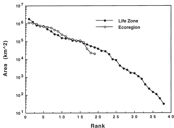
Figure 6 Rank order by area of the thirty-eight life zones of the United States and the ecological provinces of Bailey et al. (1994).
