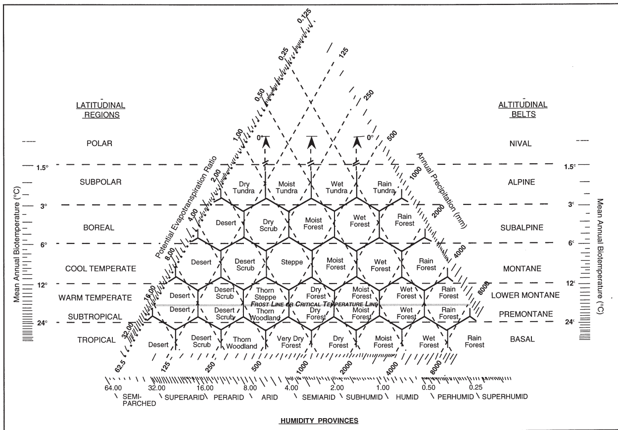
Figure 1 The life zone chart of Holdridge (1967). Consult text for further explanation.
